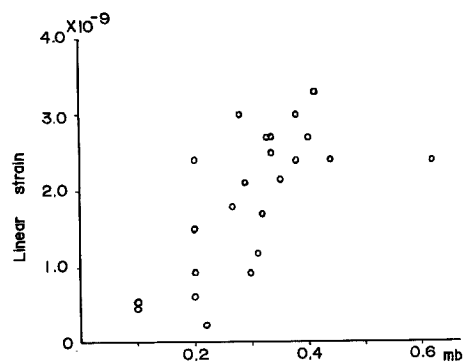
Fig. 10(b) Relation between the linear strain and pressure variation ⊙ ; Akibasan N-S component strain
