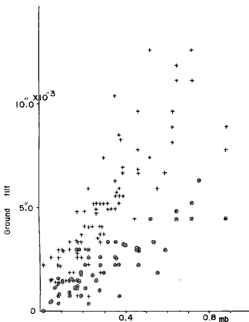
Fig. 9(a) Relations between the ground tilts and pressure variations ⊙ ; Oura E-W component tilt + ; " N-S "
