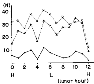
Fig. 4(a) Frequency distribution of earthquake-occurrence for the period in which semi-diurnal tides were predominating
