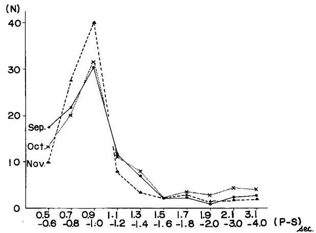
Fig. 2 Frequency distribution of P-S at Oura (Sept.-Nov., 1960)
