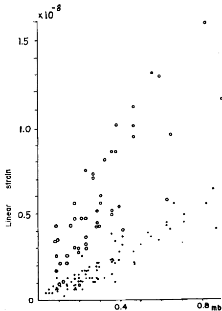
Fig. 9(b) Relations between linear strains and pressure variations ⊙ ; Oura N-S component strain ● ; " E-W "
