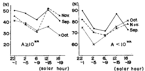
Fig. 3 Frequency distribution of time of earthquake-occurrence (Sept.-Nov., 1960)
