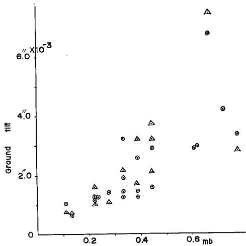
Fig. 10(a) Relations between the ground tilts and pressure variations ⊙ ; Akibasan E-W component tilt (Tilt-meter with damper) △ ; Akibasan W-E component tilt (Tilt-meter without damper)
