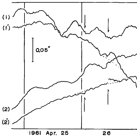
Fig. 13 Remarkable local earthquakes on Apr. 26, 1961 (1) ; Akibasan E-W tilt (original) (1') ; " (corrected) (2) ; Akibasan N-S tilt (original) (2') ; " (corrected) ↓ ; Remarkable local earthquake
