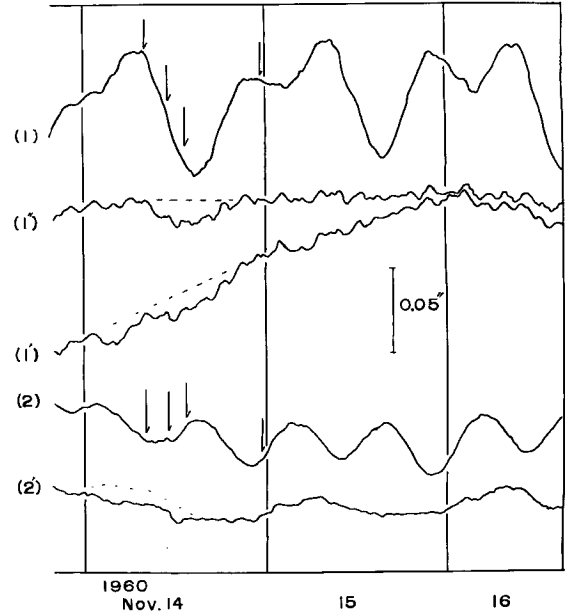
Fig. 14 Remarkable local earthquakes on Nov. 14, 1960 (1), (2) ; original (1'), (1''), (2') ; corrected
