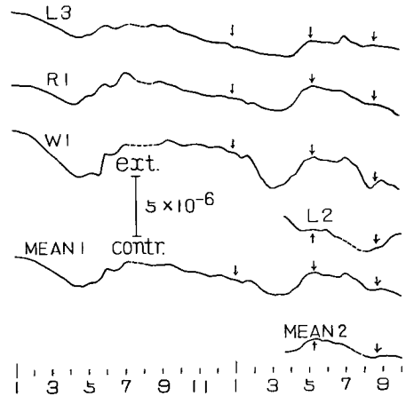
Fig. 3 Observed curves of the linear strains in the direction of N38°E
