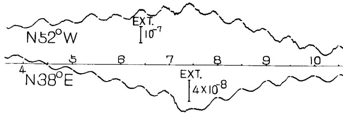
Fig. 13 (B) Recods of extensometers
