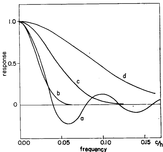
Fig. 1 Frequency response of an equally-weighted running mean and of normal probability curve smoothing function. Curve (a) is response of the 25-hour running mean. Curves (b), (c) and (d) are response of normal curve smoothing functions having 8-, 4- and 2-hour data intervals computed from equation (6), respectively.
