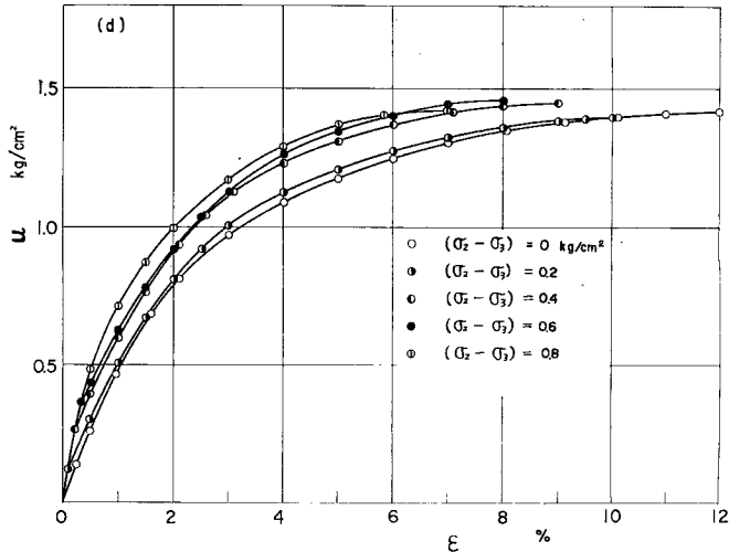
Fig. 6 (d) Pore-water pressure - strain curves ( \sigma_1 > \sigma_2 > \sigma_3 tests; \sigma_e = 2 \text{ kg/cm}^2 )
