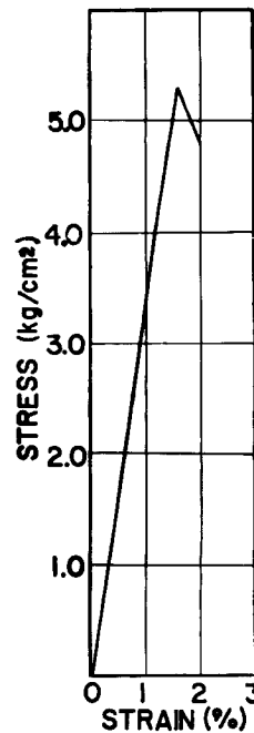
Fig. 3. Stress-strain curve.
