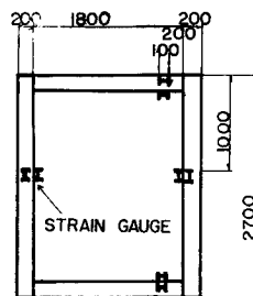
Fig. 1. H-shape support.
