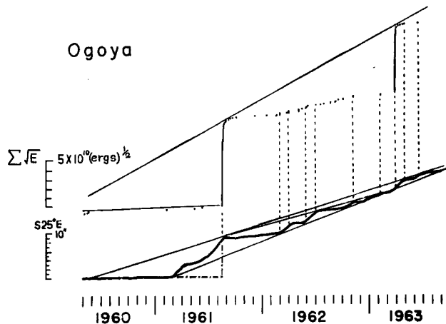
Fig. 5. Tilt variation (Lower) in the direction of horizontal displacement, added the constant rate of 7"/year to the real secular variation for comparison with the state of energy release (upper) caused by the earthquakes of sequence B.
