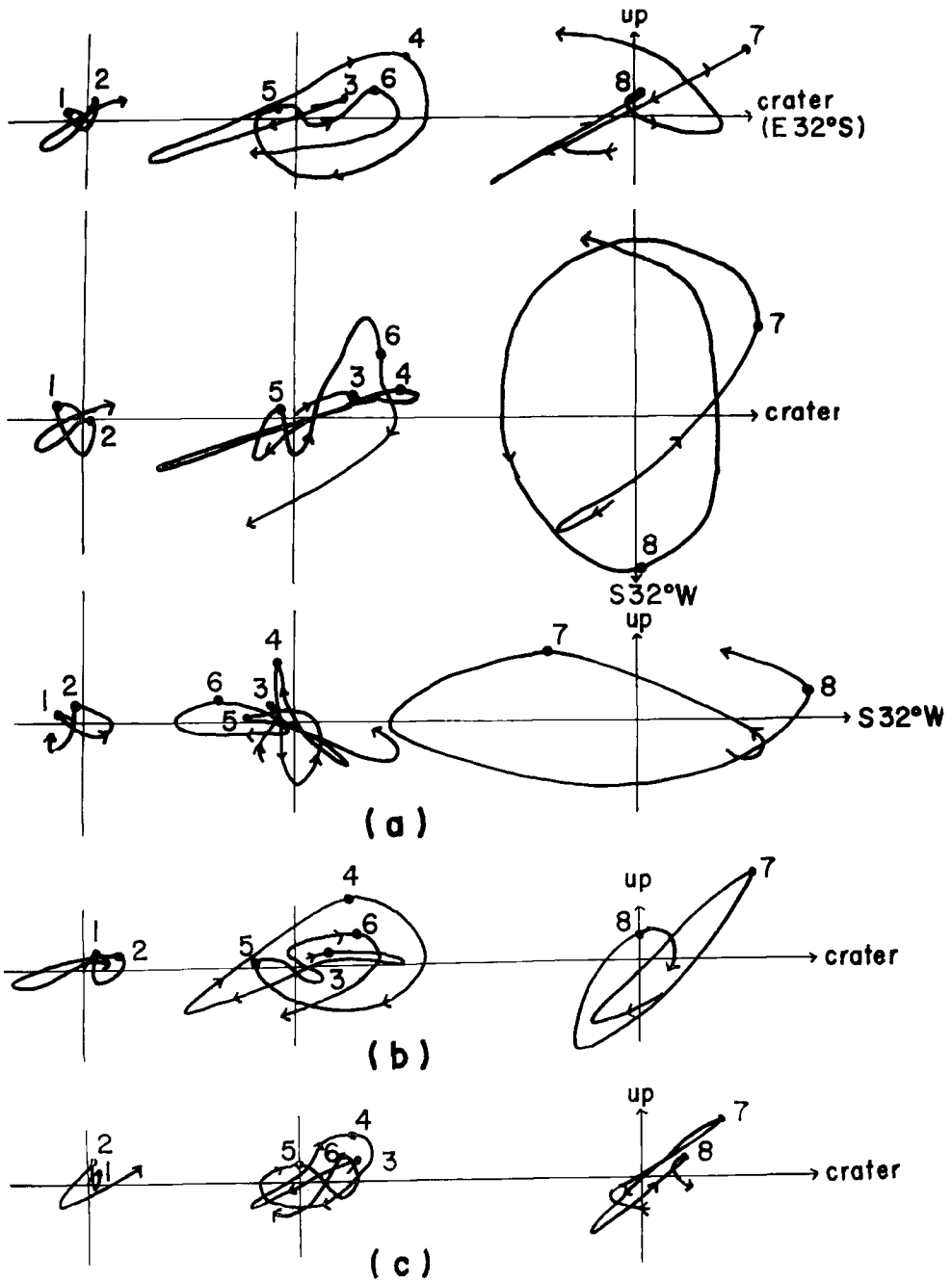
Fig. 5. Wave-orbit diagrams of volcanic earthquake in Z-crater plane at three observing sites of Harutayama and Kurokami. (b) in Kurokami's diagrams are the smoothed ones from the original (a).
