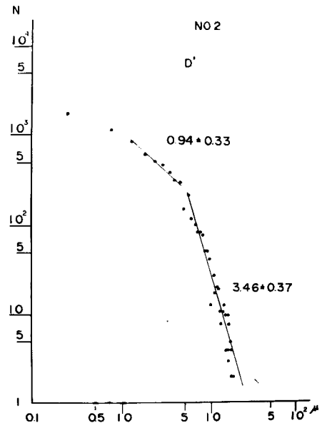
Fig. 8 Amplitude and frequency relation of volcanic micro-earthquakes of D' type at Hikino-hira station.
