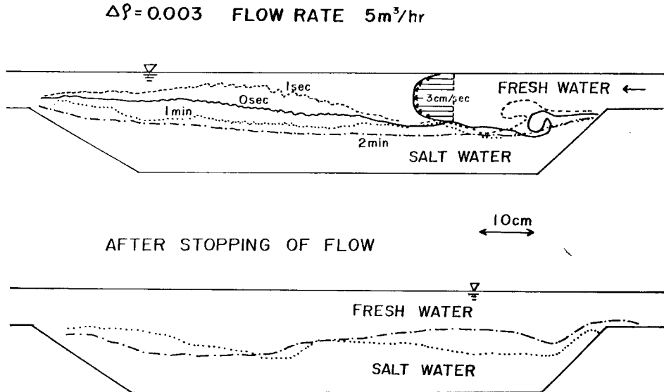
Fig. 5 Inclination of interface between fresh and salt water by the flow of upper layer and interfacial oscillation after stopping of the flow.
