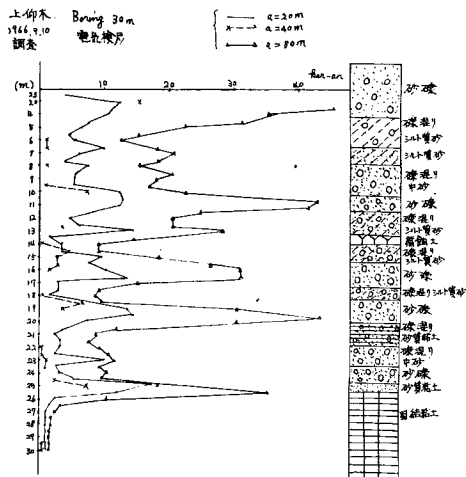
Fig. 4 Resistivity log
