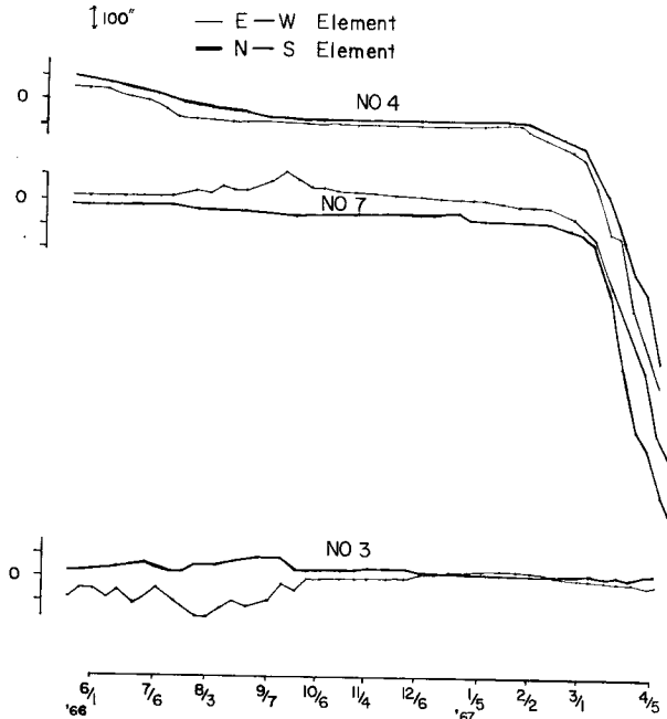
Fig. 3 The variations of the observed inclinometers at No. 4 and No. 7 during from August, 1964 to April, 1965.
