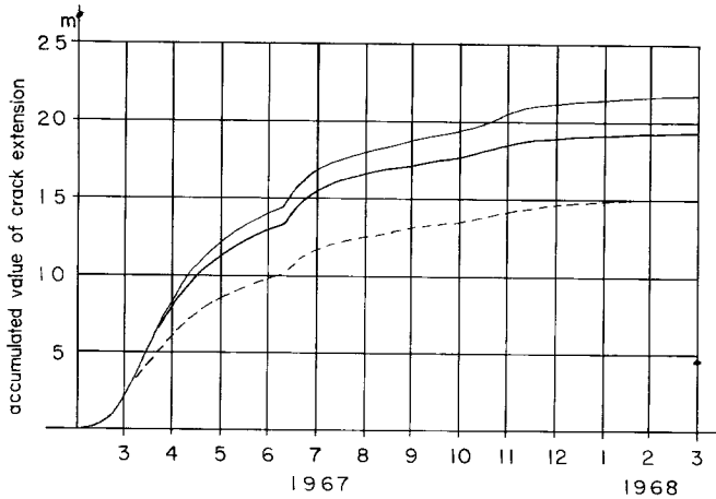
Fig. 4 The accumulated values of extension crack at Kamenose, Inlslide area.
