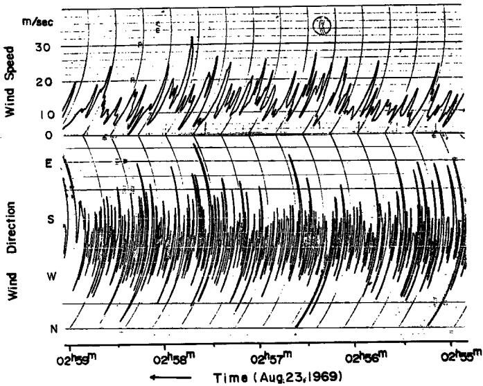
Fig. 8 Anemograph.
