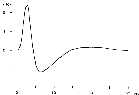
Fig. 8 Computed impulse response of the present system to the ground displacement.
