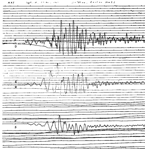
Fig. 9 Example of the three-component seismograms recorded at the Kamitakara station ( d=785 km). Epicenter: \phi=30^{\circ}.9 N, \lambda=131^{\circ}.7 E, h=40 km, M=5.5 .
