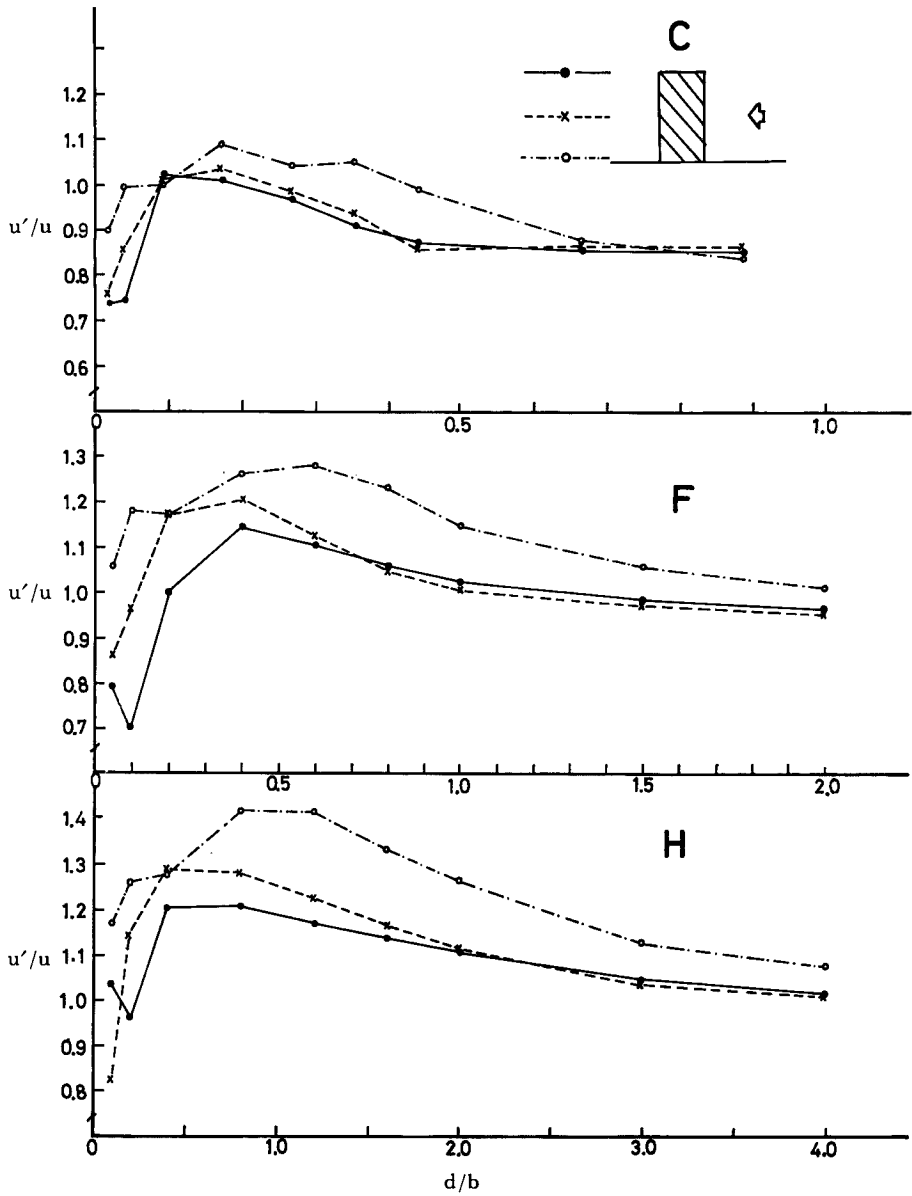
Fig. 5 Variation of reduced wind velocity with nondimensional gap width.
