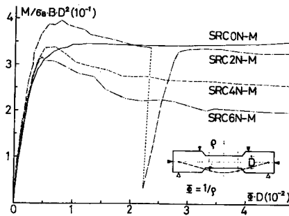
Fig. 5 Test results.
