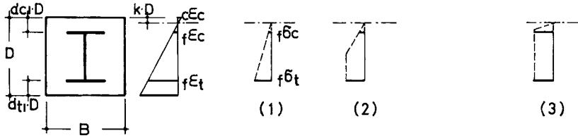
Fig. 11 Stress distribution, flange, Case 3.
