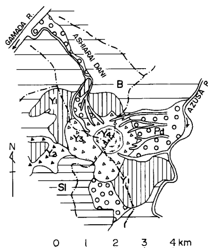
Fig. 13 Geological map of the Yakedake volcano B : Basement rocks, Y1 : Yakedake lower lava, Y2 : Yakedake avalanche breccia Y3 : Yakedake pyroclastic deposits, Y4 : Yakedake lava dome Pd : Pyroclastic flow deposits
