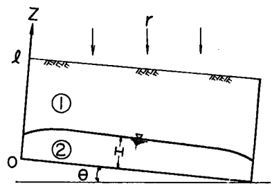
① Unsaturated zone ② Saturated zone Fig. 10 Co-ordinate system and symbols
