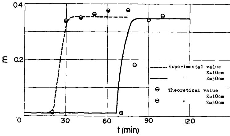
Fig. 11 Comparisons between theoretical values and experimental curves; Exp. No. A-1
