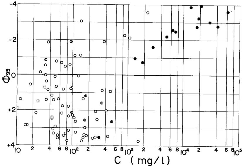
Fig. 2 Relation between C and \phi_{95} . Darkened circles are data on 8 August and halbed on 29 June.
