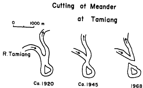
Fig. 6 Change in River Course at Rantau. (North Sumatra)
