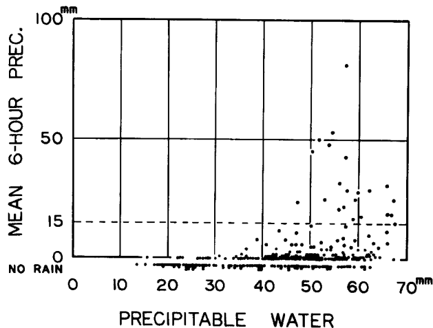
Fig. 2 Relation between mean humidity and mean 6-hour precipitation.
