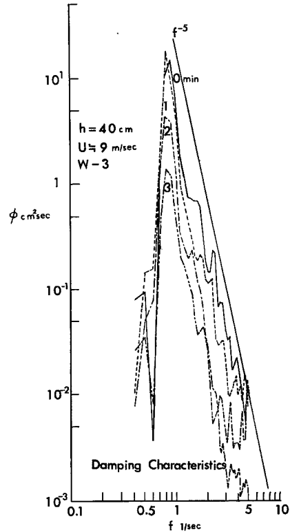
Fig. 16 Damping characteristics of wind wave spectra.
