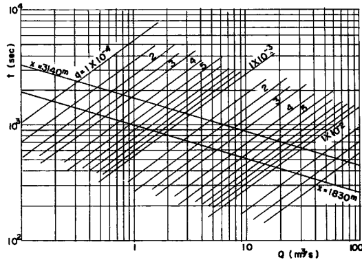
Fig. 11 Figures for t = KQ^P/q in upper sub-basin, Model B. In which, t is time (sec), Q is discharge in river ( m^3/sec ), q is inflow discharge for unit length of the river ( m^2/sec ), K and P are constants.
