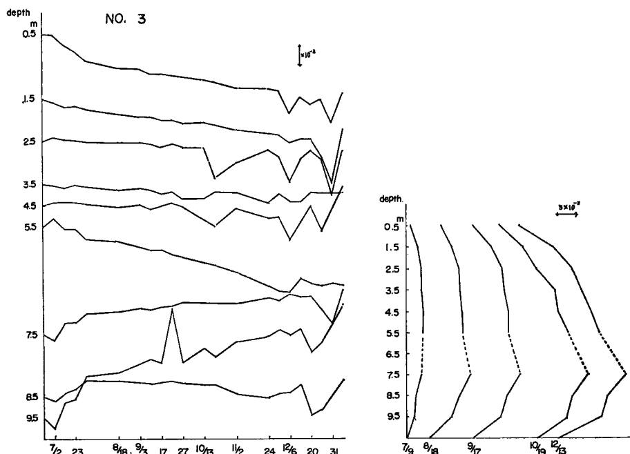
Fig. 4a Variations of internal strain and accumulated internal strain at No. 3.
