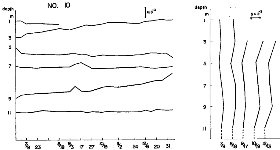
Fig. 4 e Variations of internal strain and accumulated internal strain at No. 10.
