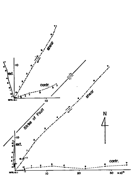
Fig. 7 Secular changes of the principal axis of strain at each side of the fault.
