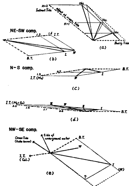
Fig. 15 Resolution of the observed tidal oscillation.
