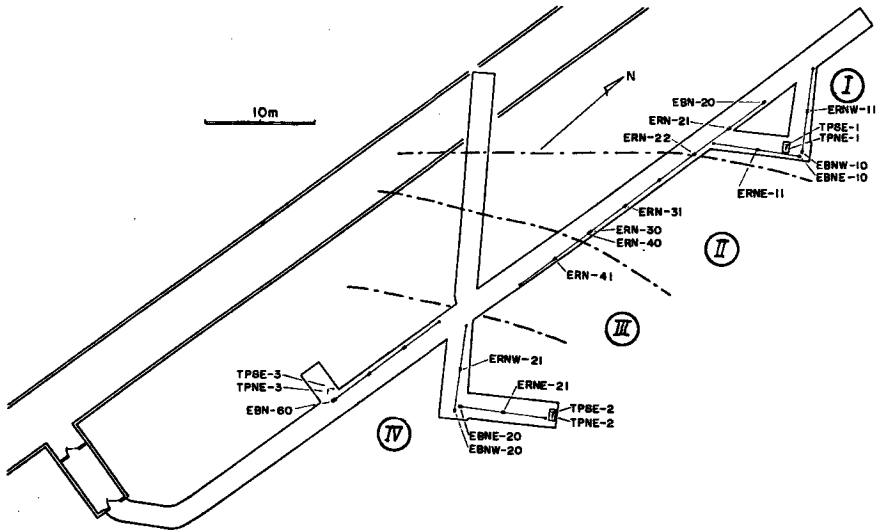
Fig. 1 Arrangement of instruments for preliminary observation.
