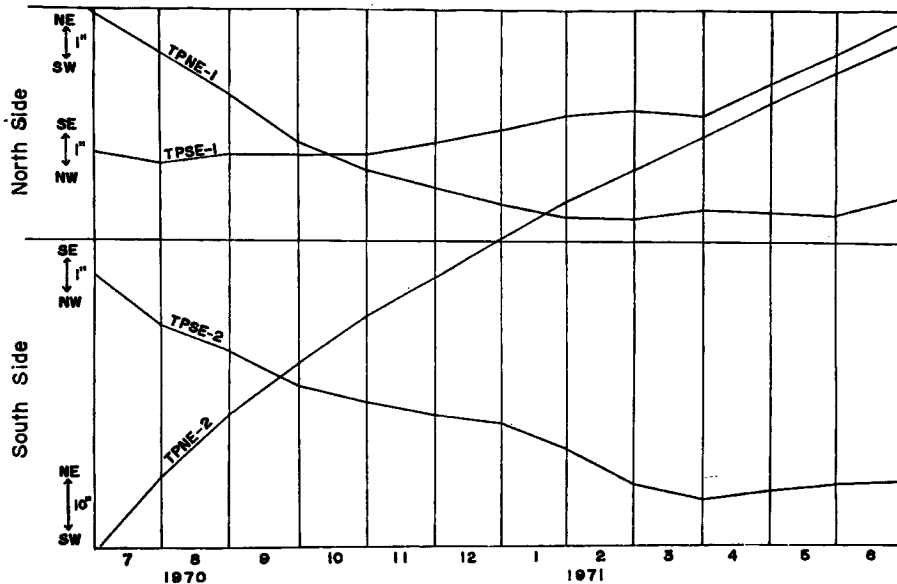
Fig. 10 Secular change of ground tilts observed at the north and south sides of the Ootsuki fault.
