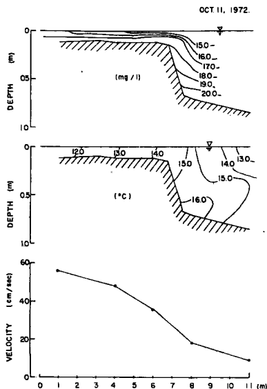
Fig. 14 Longitudinal profiles of turbidity, water temperature and flow velocity in the mouth of Fujinoki river, on October 11, 1972.
