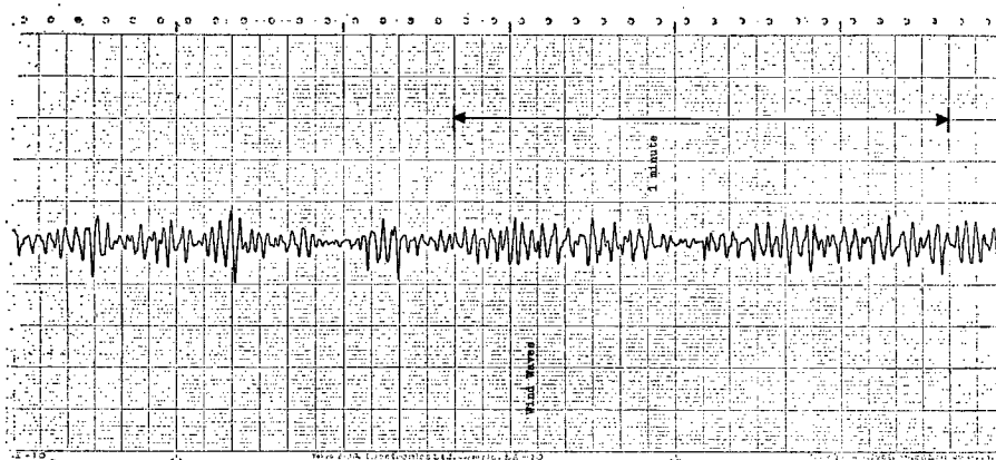
Fig. 15 (a) An example of the record of wind waves obtained by wave-level meter at the Fujinoki delta.
