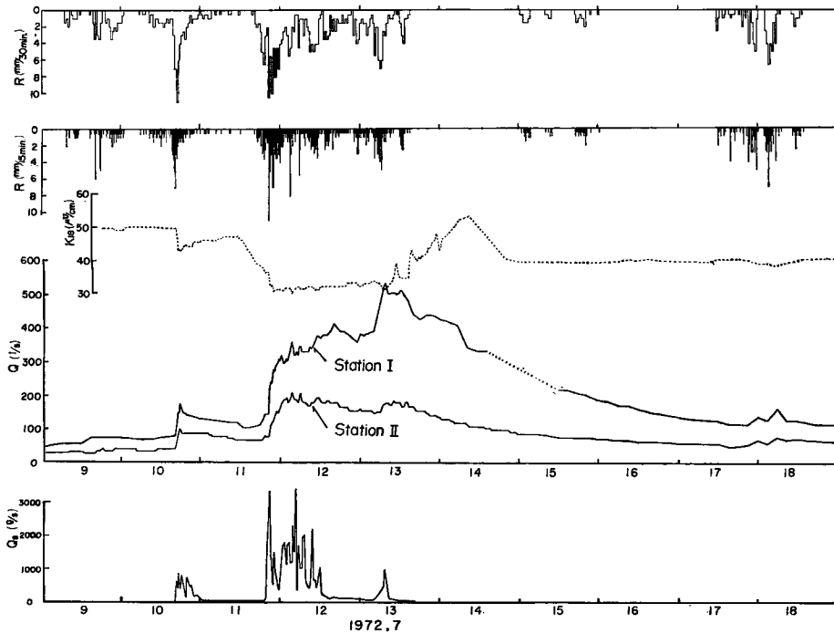
Fig. 3 Variations in discharge, sediment discharge, rainfall, and conductivity of river water during flood.
