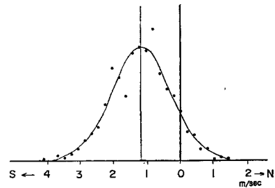
Fig. 2 Distribution of N-S component of wind velocity (Ooi, 1970).
