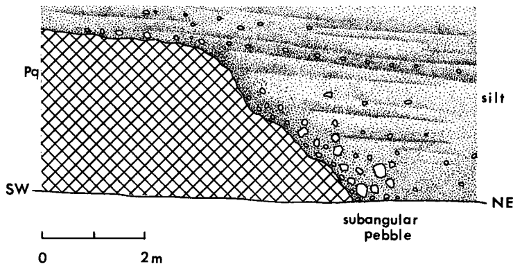
Fig. 15 Schematic sketch of an unconformity represented by overlapping of the Kobiwako Group on quartz-porphyry in the north of Katada.
