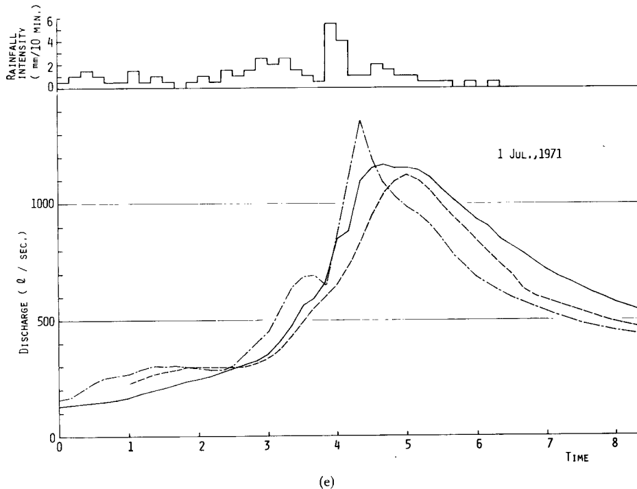
(e) Fig. 5 (a) (b) (c) (d) (e) Comparison between observed and calculated hydrographs. Full line and broken line show the observed and calculated hydrographs, respectively, and chain line the hydrograph observed in Ara experimental basin used as unit basin in the calculation.
