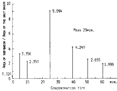
Fig. 4 Time-area-concentration diagram.
