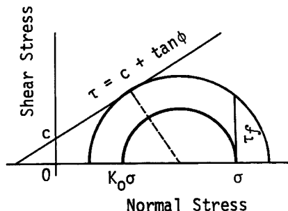
Fig. 4 Shear strength.
