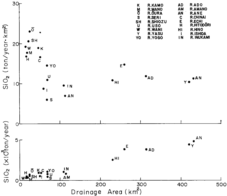
Fig. 4 Plots of SiO 2 transport rate against drainage area of rivers around Lake Biwa.
