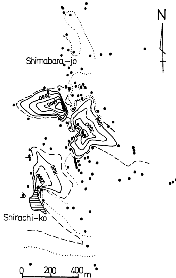
Fig. 2. Distribution map of the quantity of well water in the lake Shirachi and it's environs. (unit of numbers= m^3/day )
