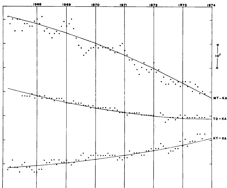
Fig. 2. Secular changes of differences of the total intensity among Tottori, Memambetsu, Kanoya and Kakioka.
