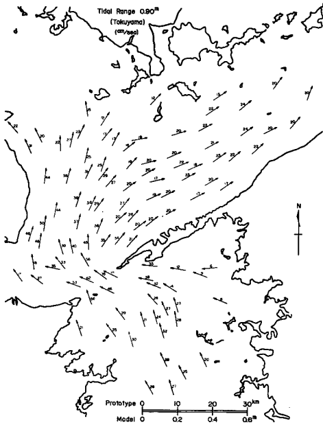
Fig. 12 Flow pattern in the flood (model, neap tide).
