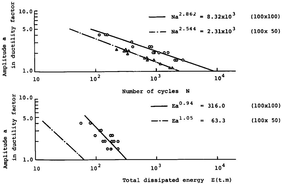
Fig. 7 SN curves and SE curves for plastic bending fatigue tests
