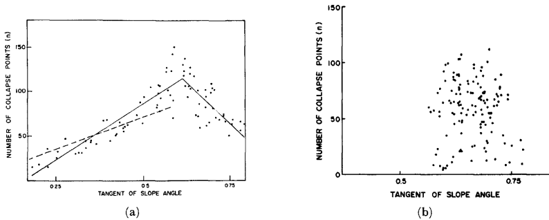
Fig. 8. Relation between number of collapse points per 2 km×2 km and tangent of slope angle (average gradient in the same square). (a): A section, (b): B section.
