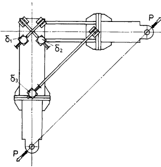
Fig. 3. Deformation instrumentation.
