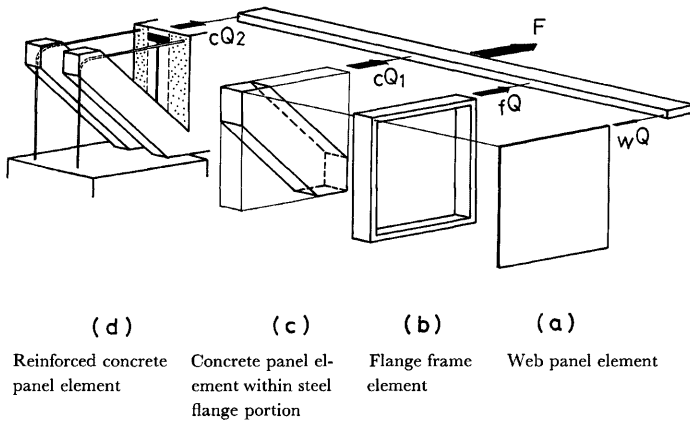
Fig. 15. Analytical model of SRC beam-to-column connection.
