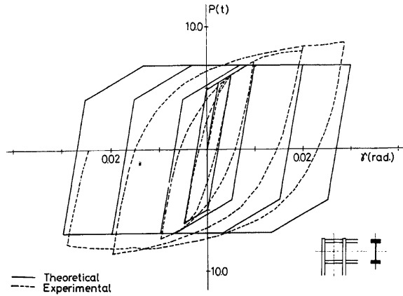
(a) Specimen L-A0R
