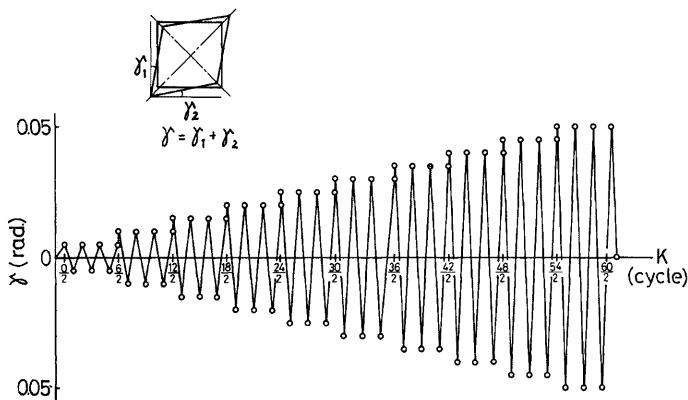
Fig. 5. Loading program.
