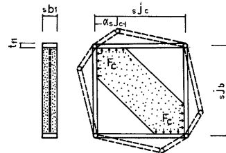
Fig. 18. Failure mechanism of concrete panel within steel flange portion.
