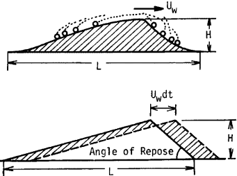
Fig. 20. Sketch of sand movement and marching of sand wave.
