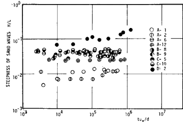
Fig. 19. Time variation of steepness of sand waves.
