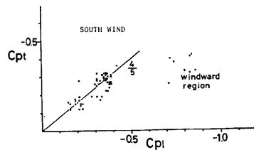
Fig. 17. The comparisons of the mean wind pressure coefficients between smooth and turbulent wind tunnel tests. (South wind)
