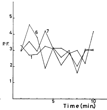
Fig. 7. Peak factors of the wind pressures at NE-corner of the roof. (2)
