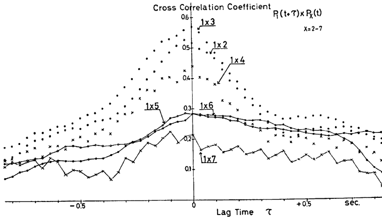
Fig. 10. Cross correlation coefficients between the wind pressurer fluctuations at NE-corner.
