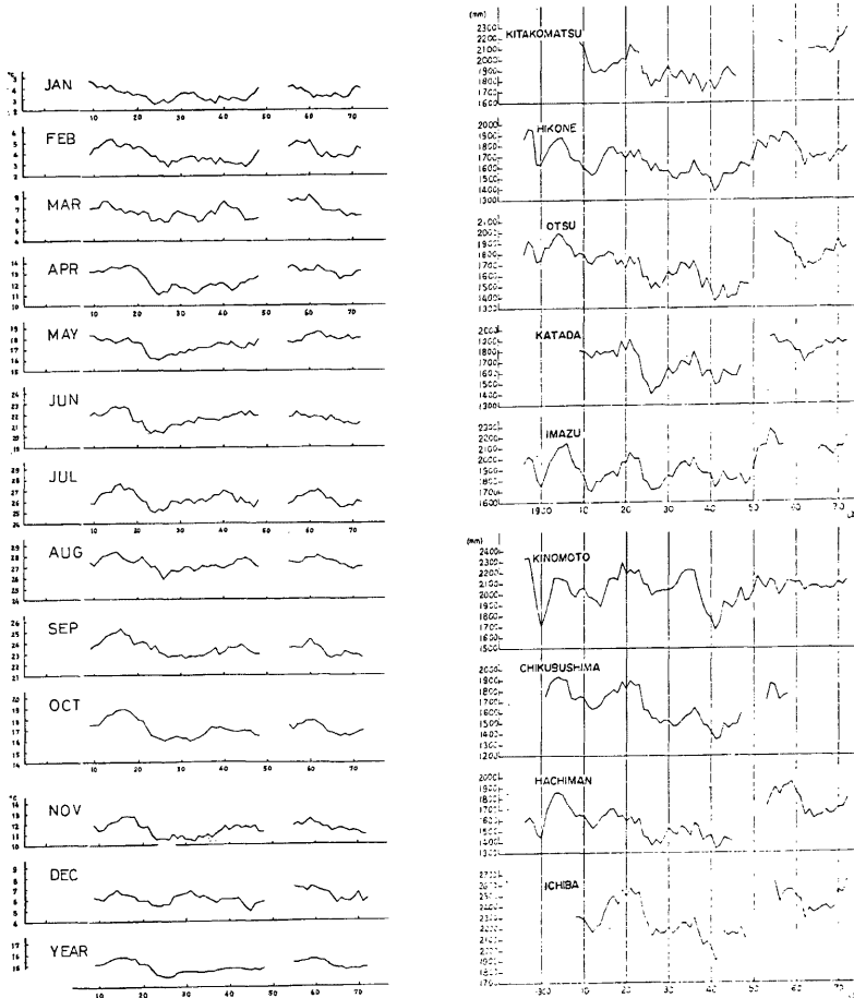
Fig. 8. Change of annual rainfall amounts of 9 stations around Lake Biwa. (5 years running mean)
