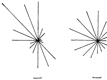
Fig. 4. Wind rose at Hikone on January for 1895-1945. Left: Frequency of occurrence. Right: Mean wind velocity. Unit indicated at the bottom of the figures are 100 hours and 1 m/s.
