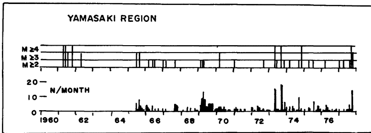
Fig. 3. Time series of seismic activity in the Yamasaki fault area. The upper and lower are due to the Japan Meteorological Agency and Tottori Microearthquake Observatory, respectively.
