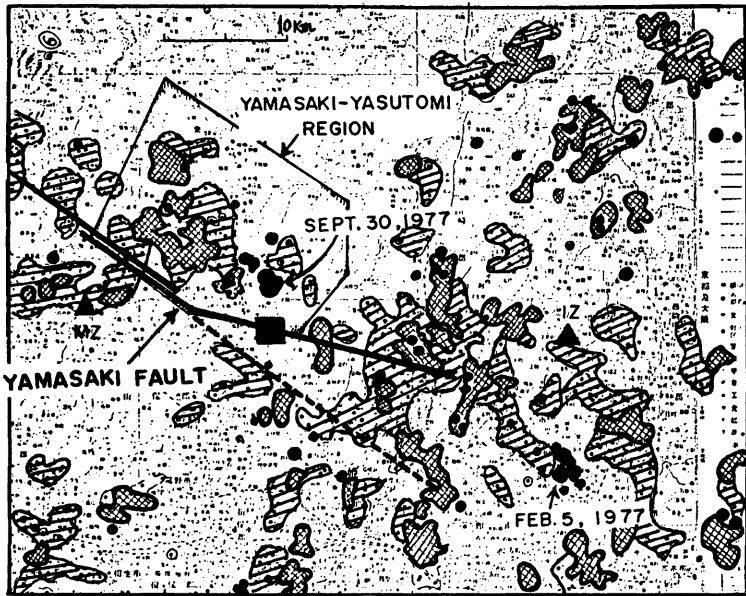
Fig. 2. Seismic activity around the central part of the Yamasaki fault. Meshed and shaded parts represent the areas which showed very high and relatively high seismicity in the past 12 years, respectively.
