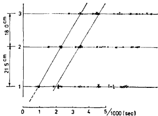
Fig. 5. Recorded accelerograms and travel time-distance curves for P-wave shot.
