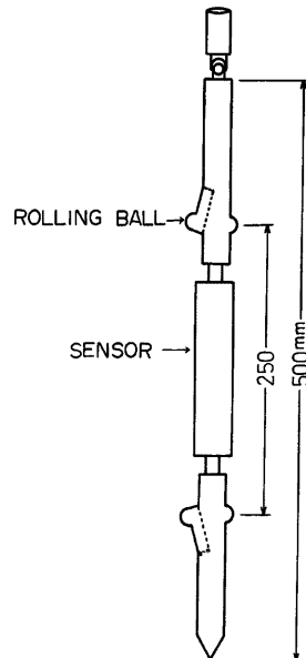
Fig. 8. In-hole inclinometer.
