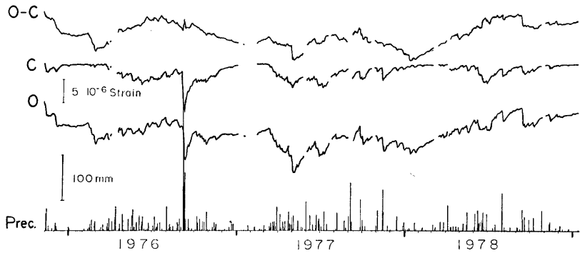
Fig. 9. Comparison between calculated strain from a tank model and observed strain (o) shows observed strain curve in which the annual change and secular change are reduced and (c) shows the calculated strain.
