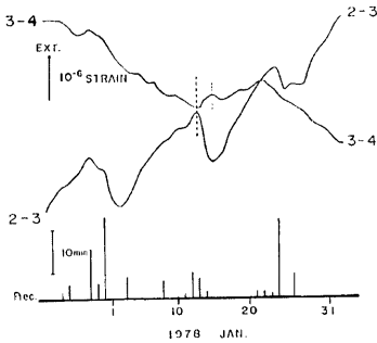
Fig. 3. Example shows the phase differences of variations caused by rainfalls. Construction began in the 2-3 component on 12th and in the 3-4 component on 14th.
