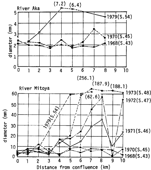
Fig. 14. Variation of mean diameter of bed materials with time and distance from confluence in the River Aka and the River Mitoya.
