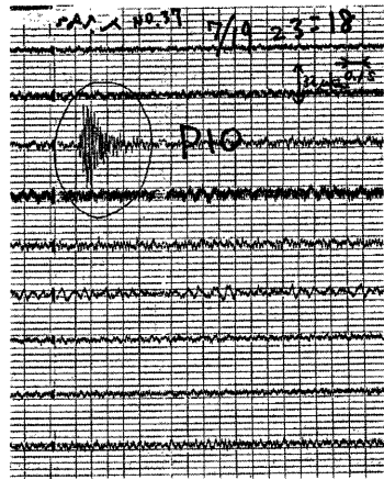
Photo. 2. Wave form of microseismic event detected at P10, whose predominant frequency is about 120 Hz.
