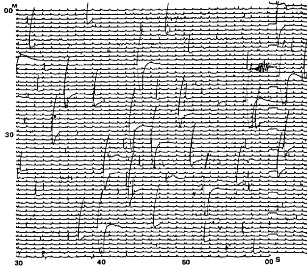
Fig. 6. Examples of usual ELF flashes recorded in a very fine day, and an example of ELF signal clearly showing a dispersion, which appear in the upper right of the record.
