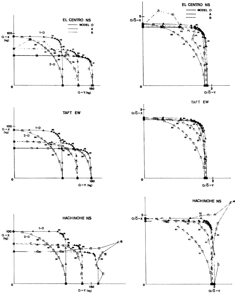
Fig. 4 Maximum shear and nondimensional maximum shear vectors of the models subjected to oblique ground motion. (□ : considering interaction, △ : without interaction)
