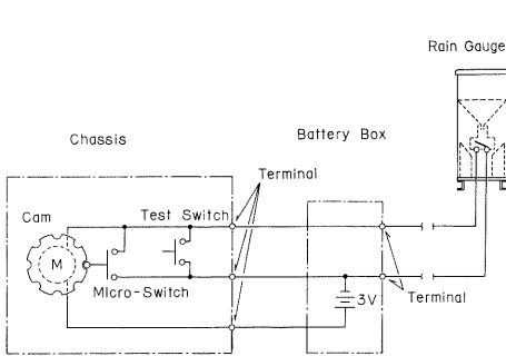
Fig. 3 Schematic diagram of the electric circuit, Type C.
